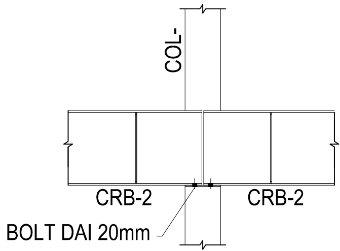
DETAIL=A-A
