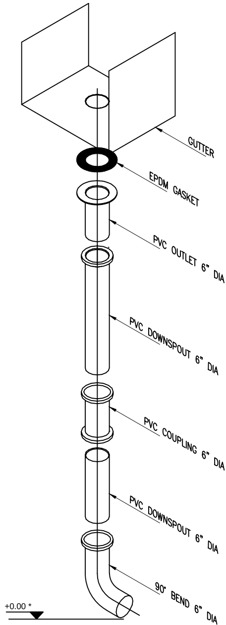
PVC DOWN SPOUT FIXING DETAIL
