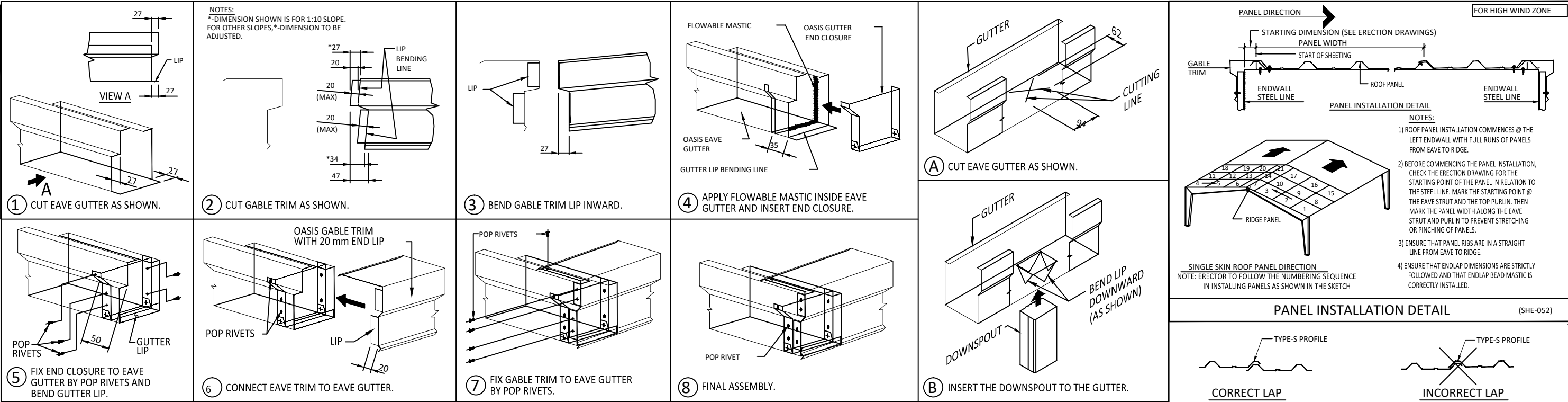
EAVE GUTTER & GABLE TRIM CONNECTION DETAIL GUTTER & DOWNSPOUT CONNECTION DETAIL
