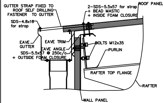
EAVE DETAIL
