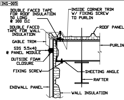
GABLE DETAIL WITH INSULATION
