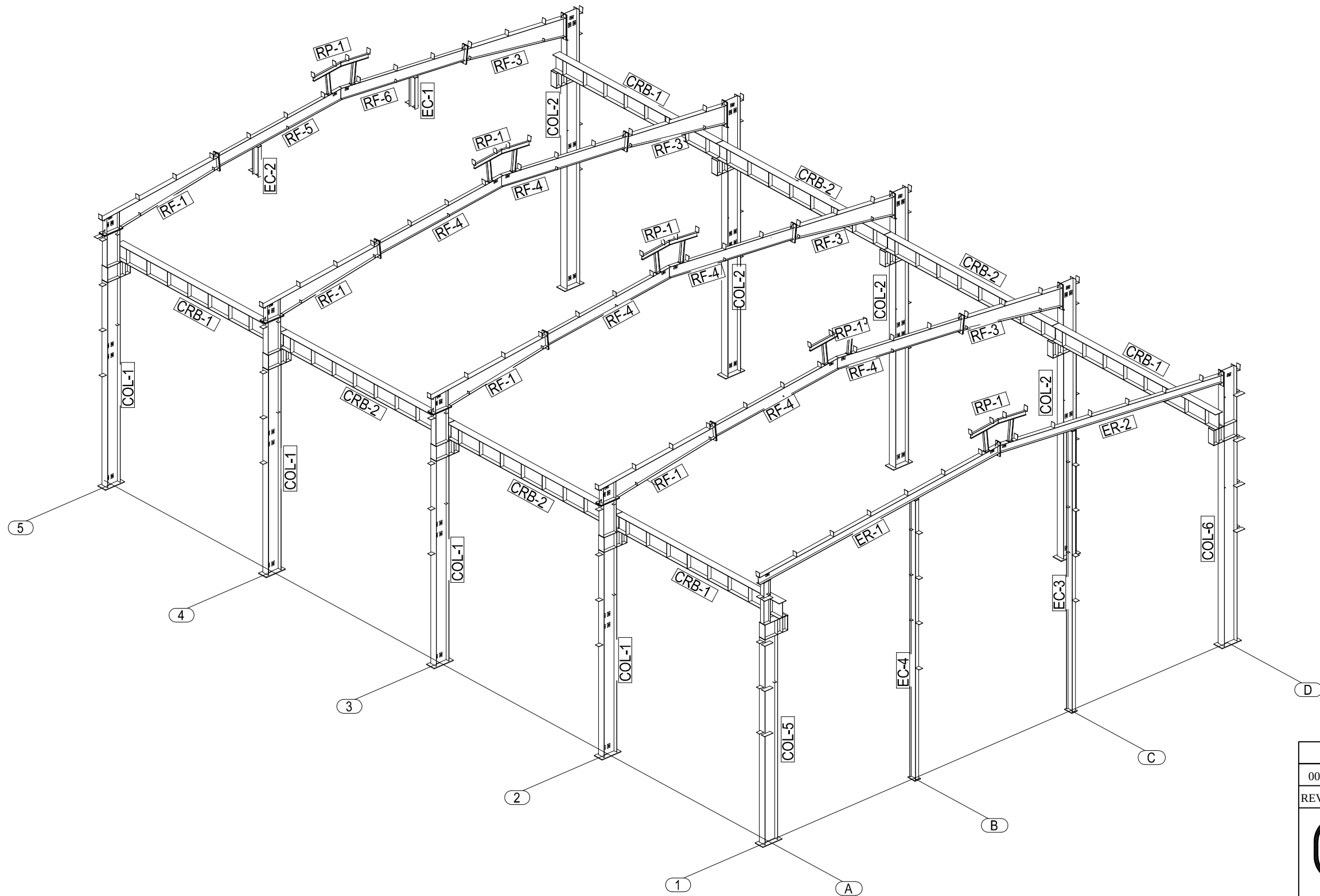
3D COLUMN AND RAFTER
