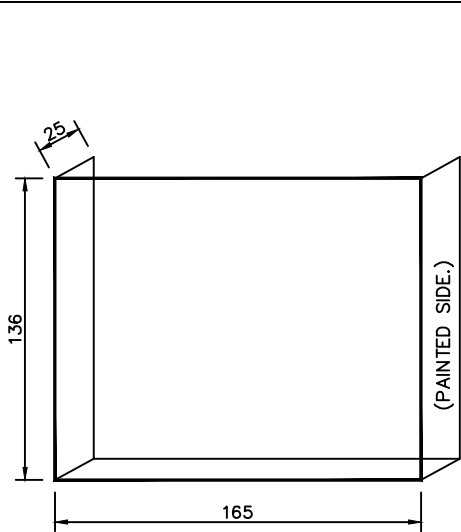
EAVE GUTTER END CLOUSURE (EC) L AND R
