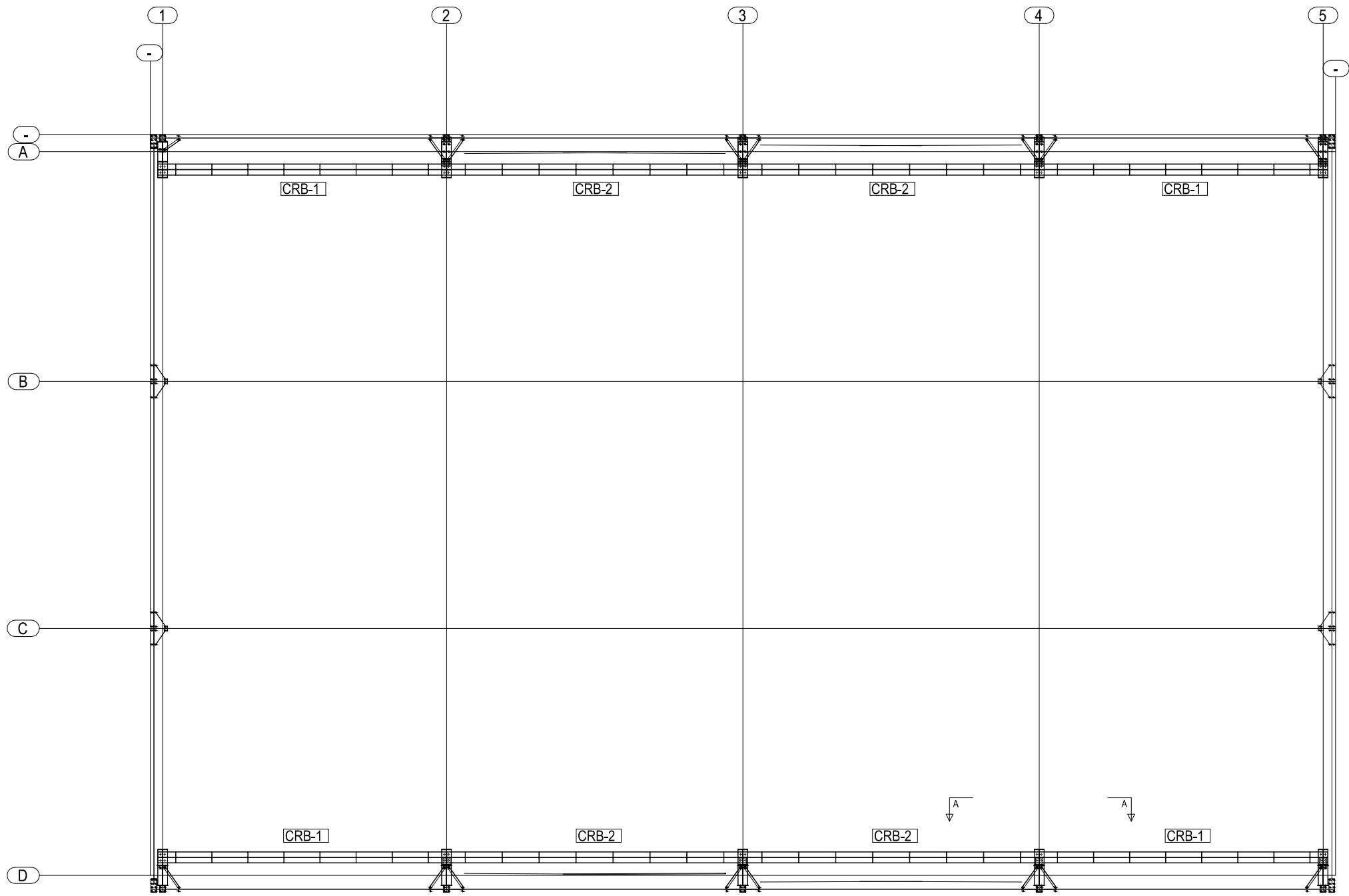
CRANE BEAM PLAN
