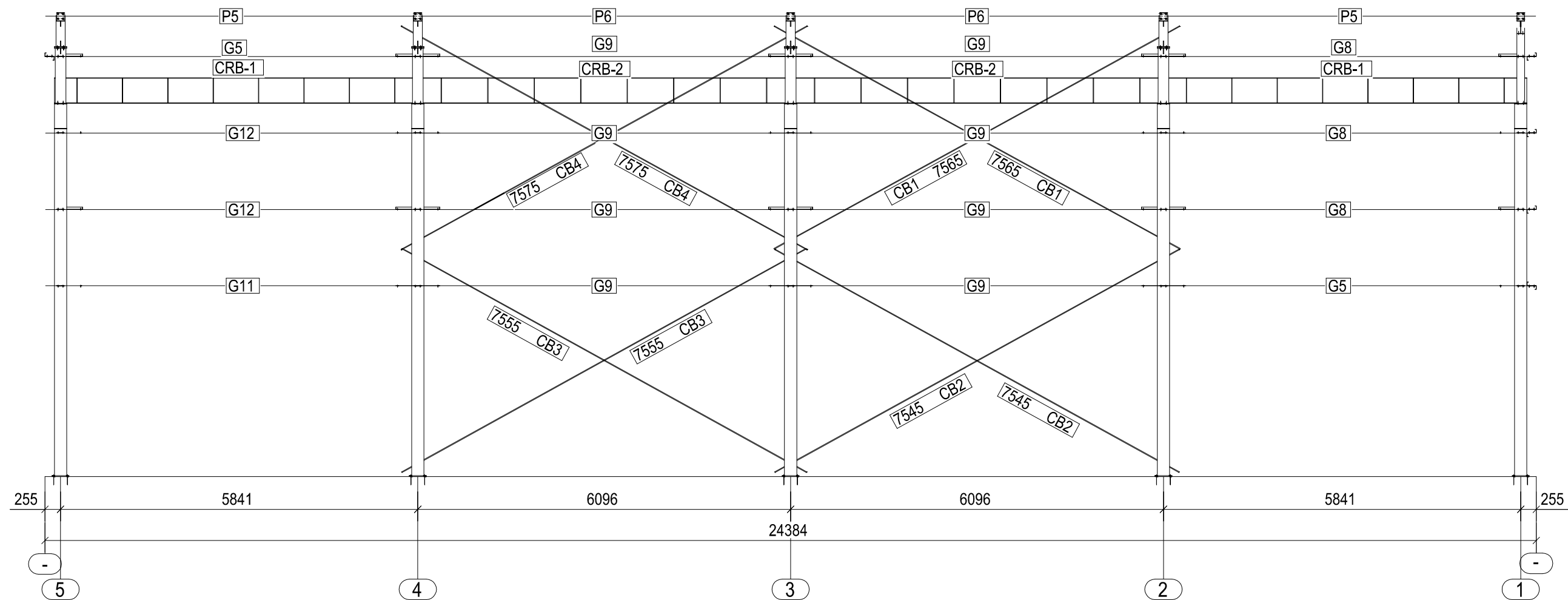
SIDEWALL ELEVATION ALONG GL-A
