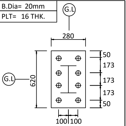
BASE PLATE DET: A
