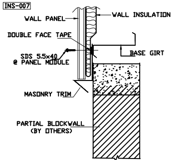
SECTION AT PARTIAL BLOCKWALL
