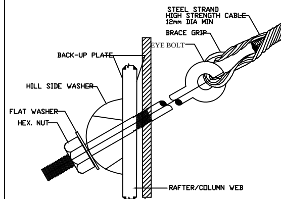
CABLE BRACE DETAIL
