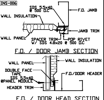
SECTION AT F.O./DOOR HEAD & JAMB
