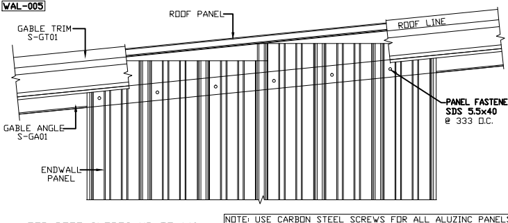
TYPICAL ENDWALL PANEL FIXING DETAIL
