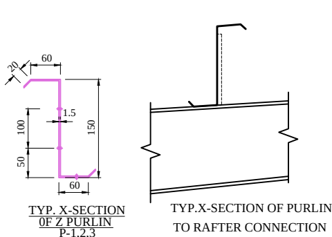
PURLIN DETAILS
