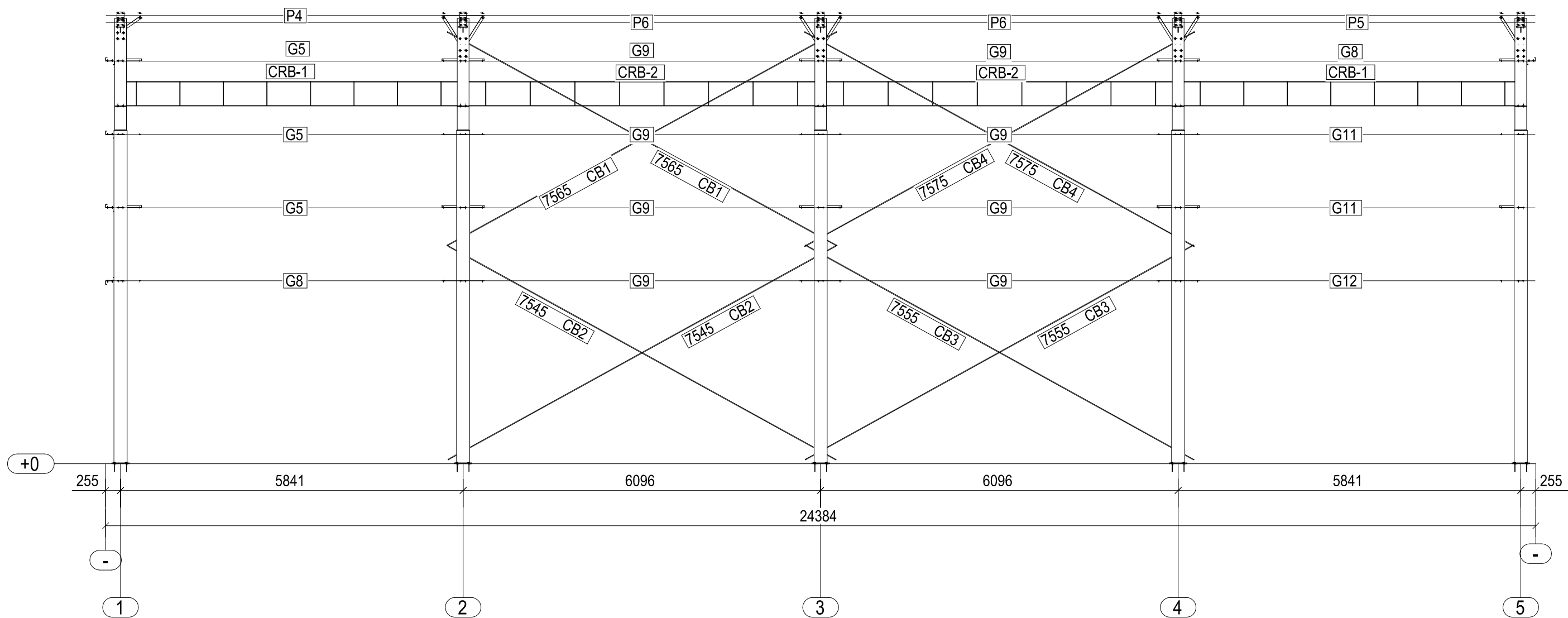
SIDEWALL ELEVATION ALONG GL-D
