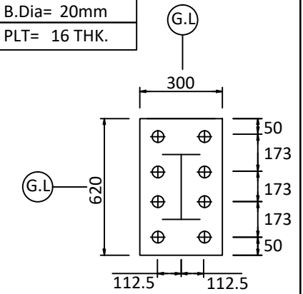
BASE PLATE DET: B
