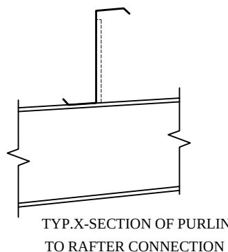
TYP. X-SECTION OF Z PURLIN P-1,2,3
