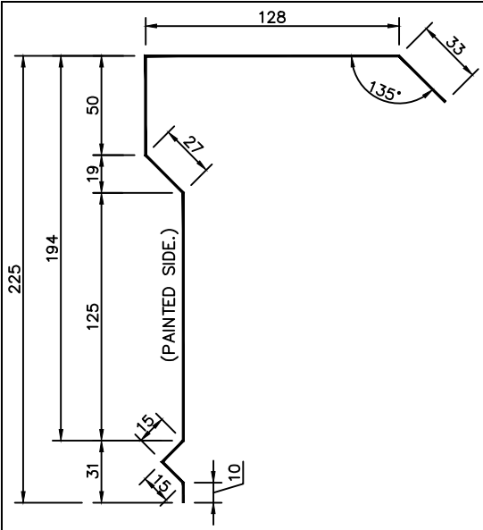
GABLE TRIM (GT)
