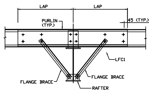
FLANGE BRACE DETAIL
