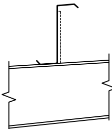
TYP.X-SECTION OF PURLIN TO RAFTER CONNECTION
