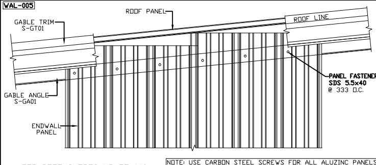
TYPICAL ENDWALL PANEL FIXING DETAIL
