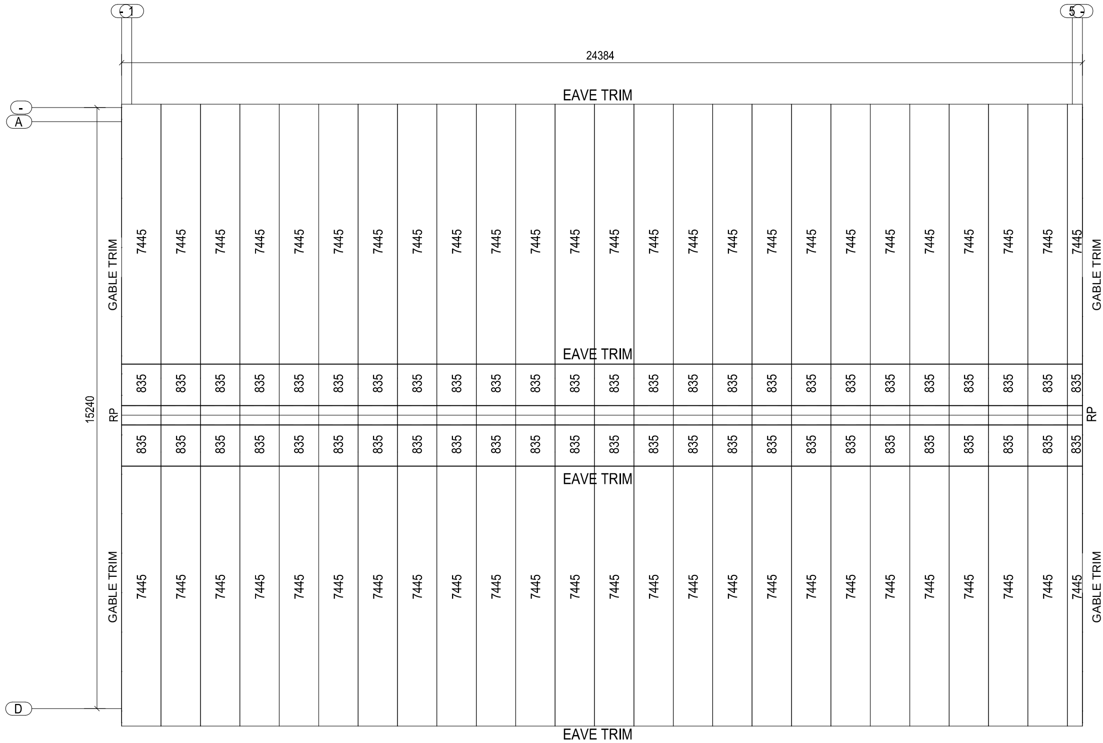
ROOF SHEETING PLAN
