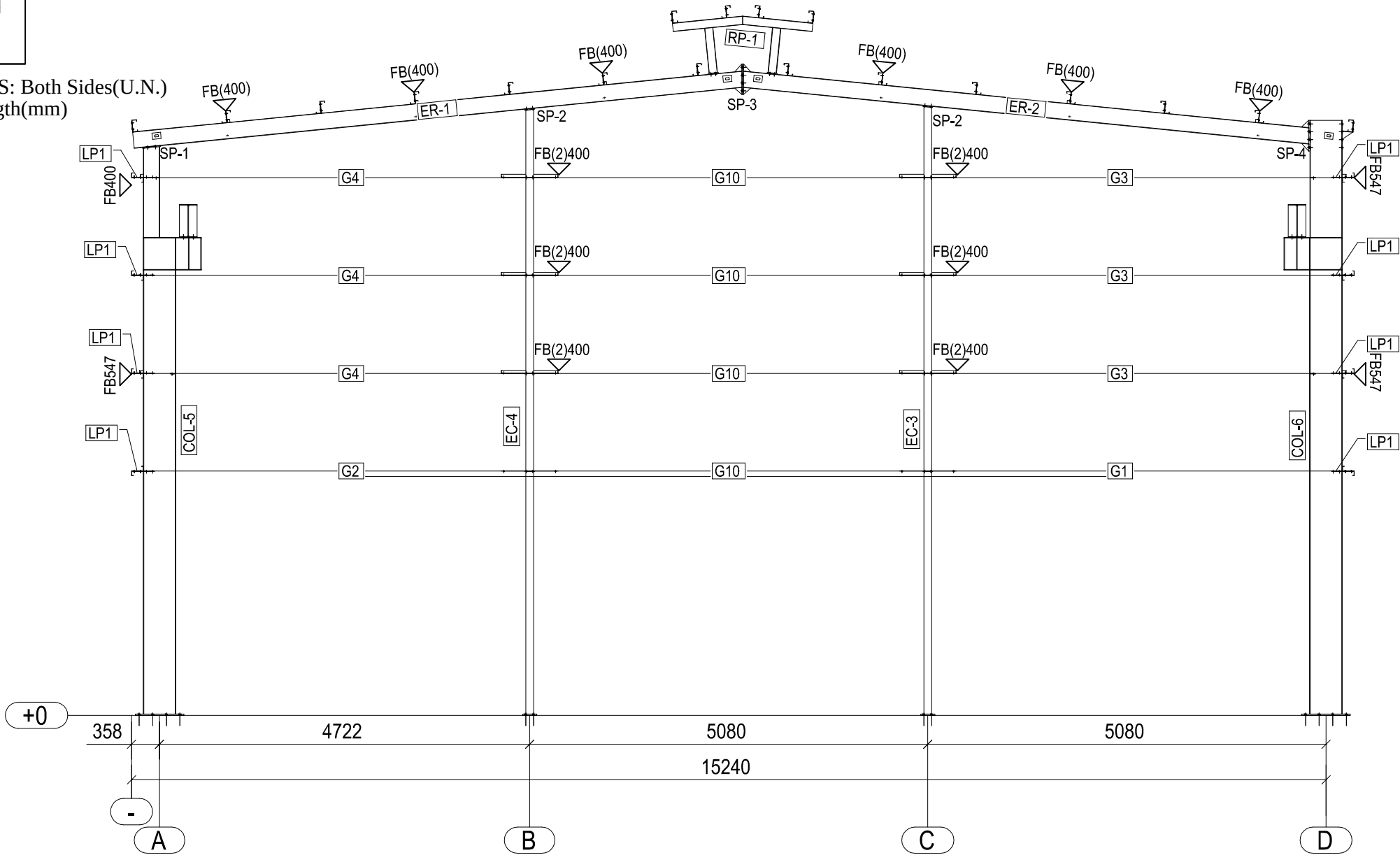
ENDWALL ELEVATION ALONG GL-1
