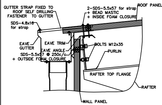
EAVE DETAIL
