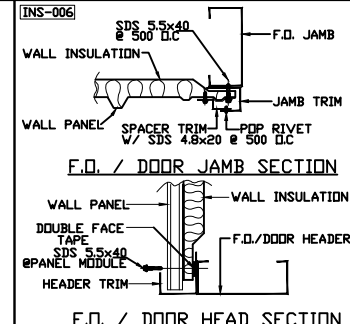
SECTION AT F.O./DOOR HEAD & JAMB
