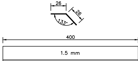
EAVE GUTTER STRAP (EGS)
