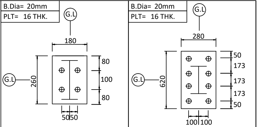
BASE PLATE DET: C
