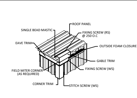
GABLE TRIM WITH EAVE TRIM DETAIL
