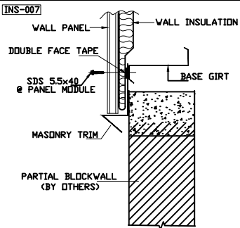
SECTION AT PARTIAL BLOCKWALL
