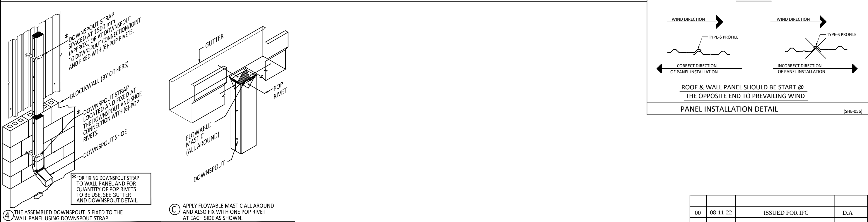
DOWNSPOUTS CONNECTION DETAIL
