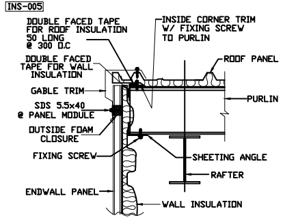
GABLE DETAIL WITH INSULATION
